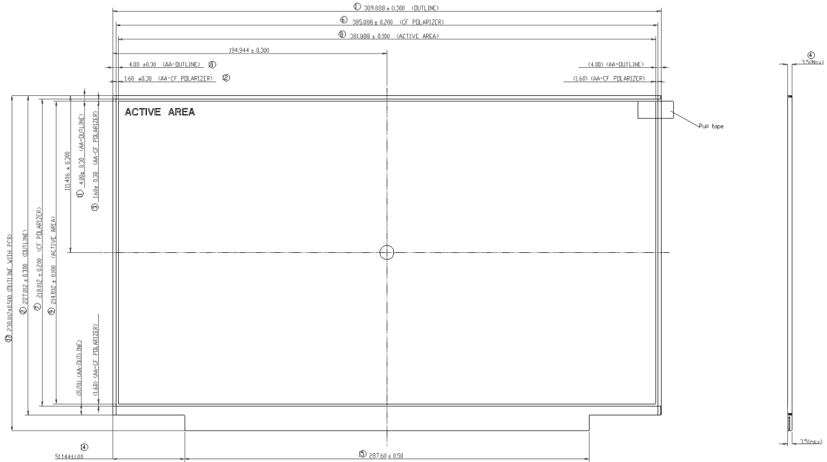
Figure 24. TFT-LCD Module Outline Dimension (Front View)
