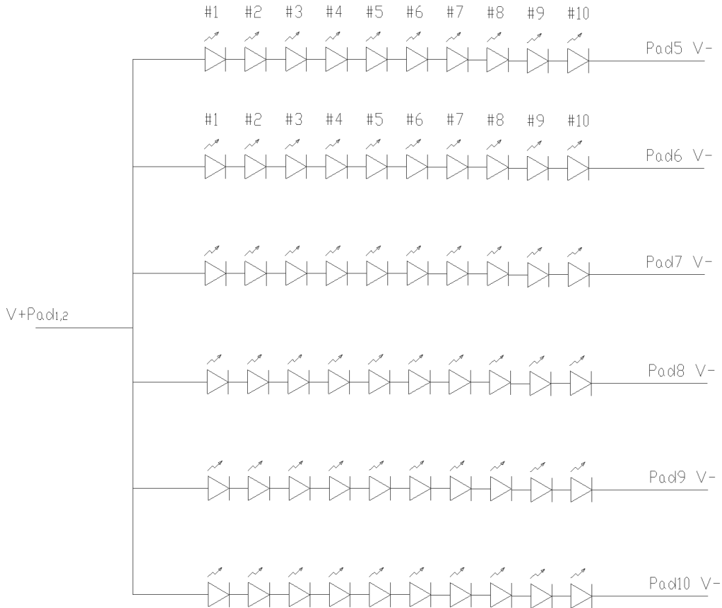
Figure 6. LED Structure
