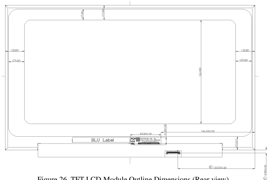
Figure 26. TFT-LCD Module Outline Dimensions (Rear view)
